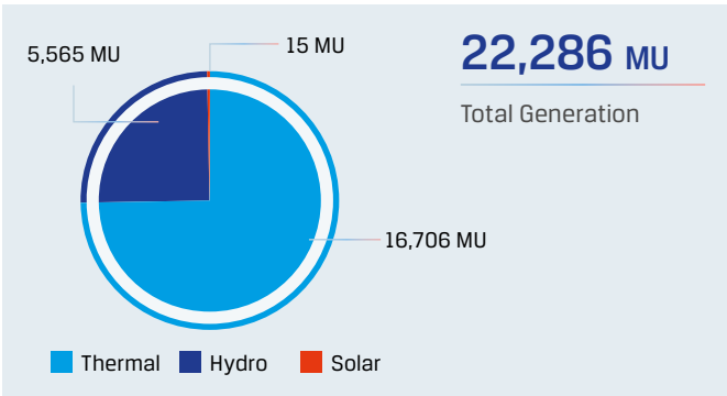
Gross Generation – By Source (MUs)
